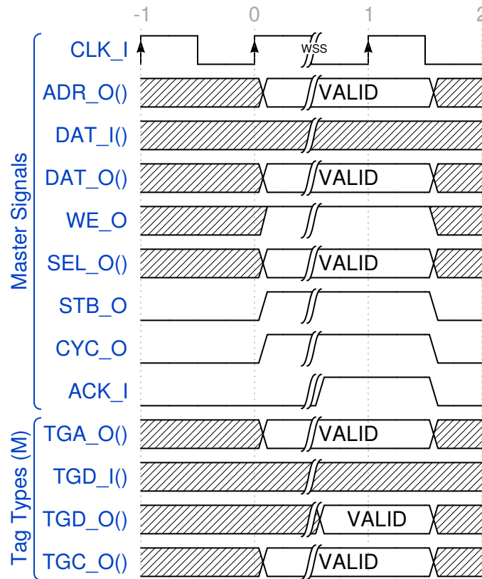
Figure 3.4: SINGLE WRITE cycle.
