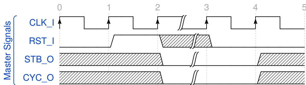
Figure 3.1: Reset cycle.
