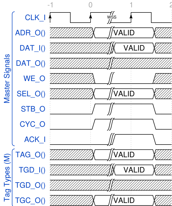
Figure 3.3: SINGLE READ cycle.
