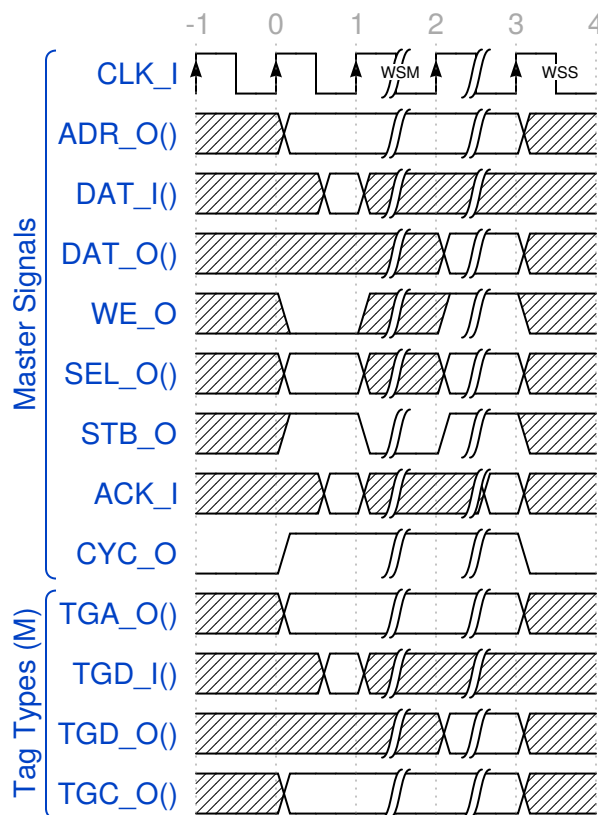
Figure 3.8: RMW cycle.
